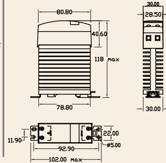
Mechanical Drawing
