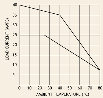
Derating Curve
